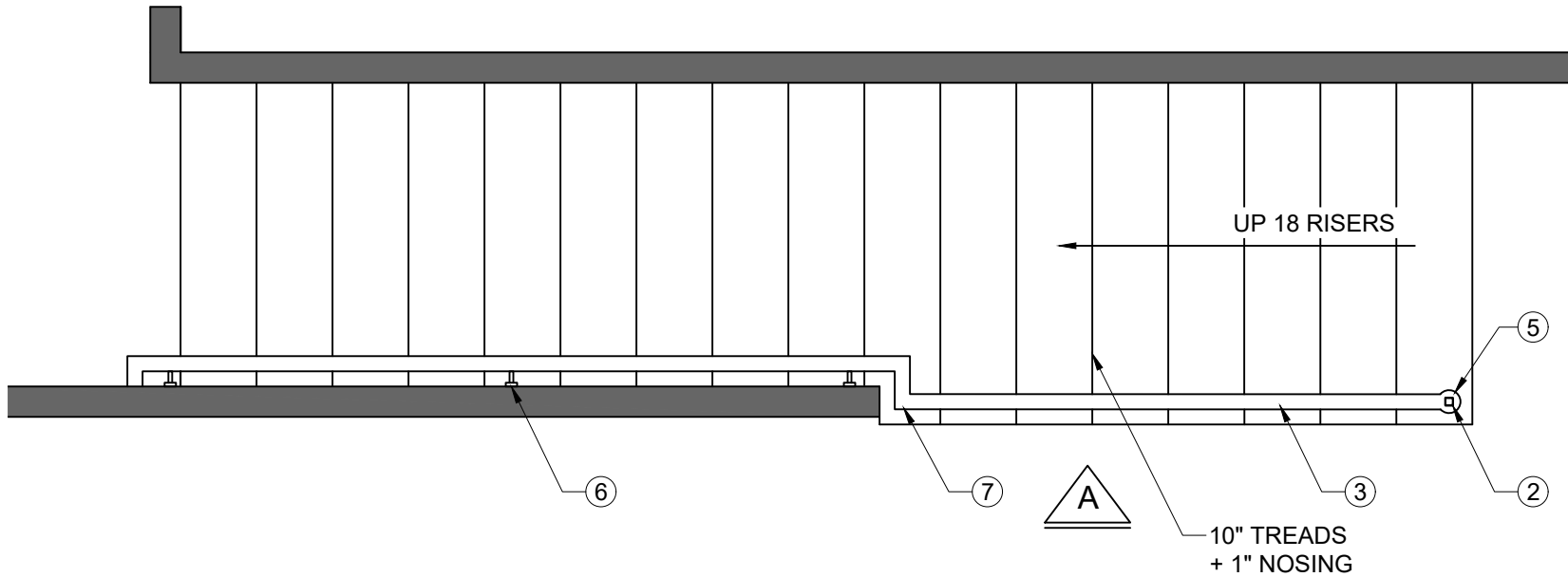
STAIR PLAN
