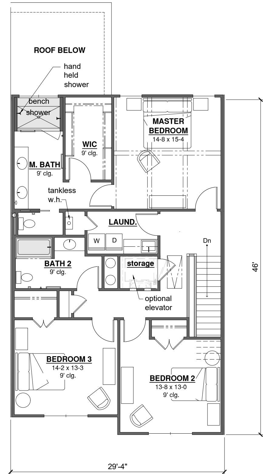
SECOND FLOOR
