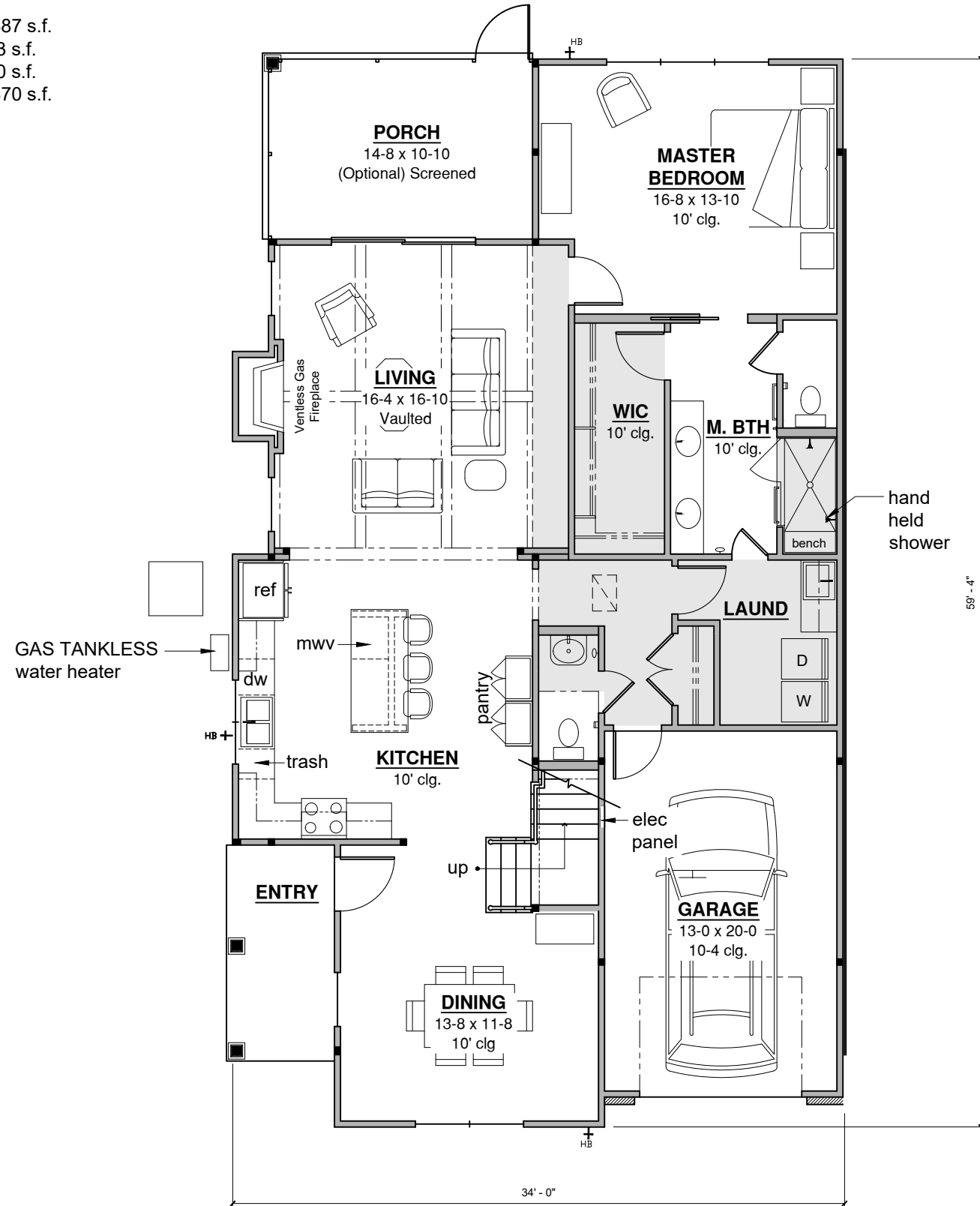
FIRST FLOOR
